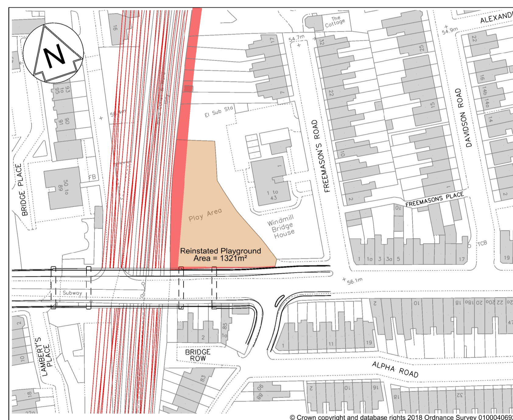
Lower Addiscombe Road/Windmill Bridge Playground Area - Proposed Operational Phase Layout
